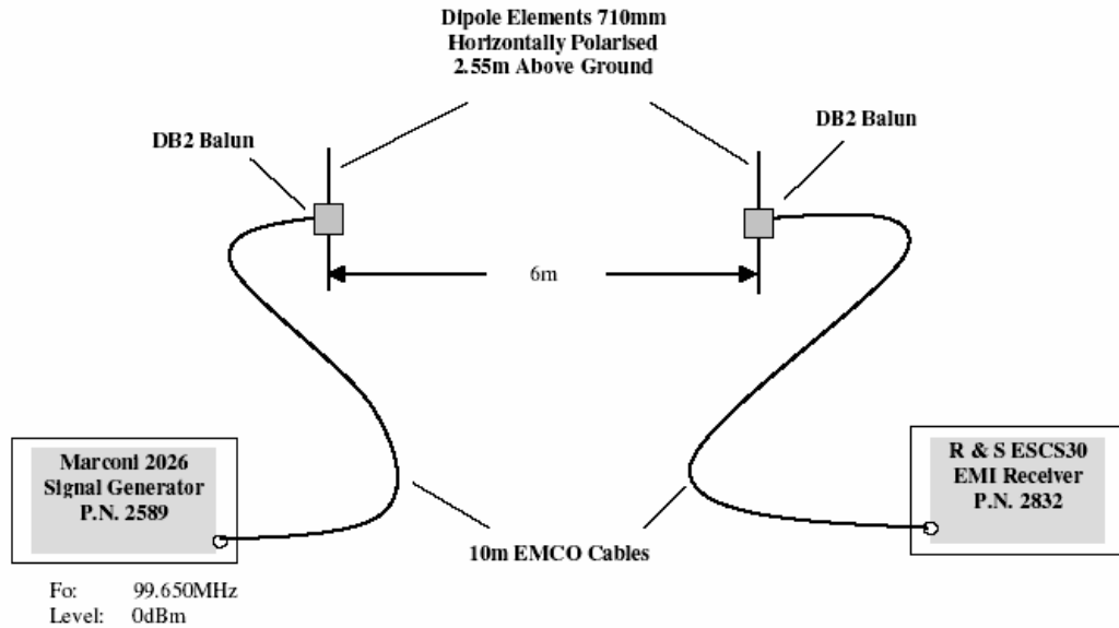
Figure 2.3: Antenna Confidence Test Setup
